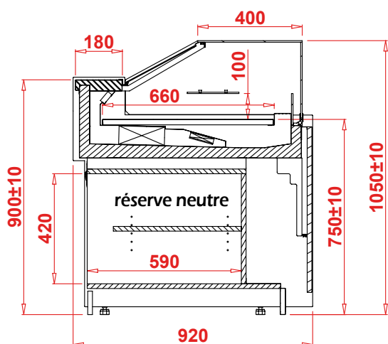
ECLAIR PA - VERSION A
